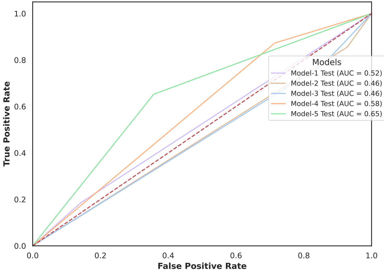
ROC Curves for Adherence Score (Test Split)
