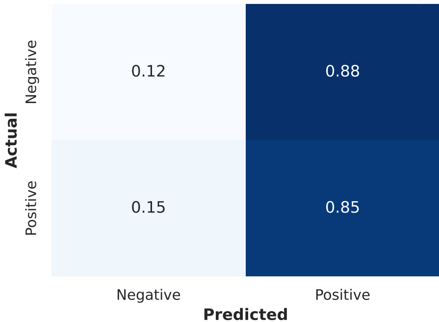
Confusion Matrix - Model-3 Val (Val Split)
