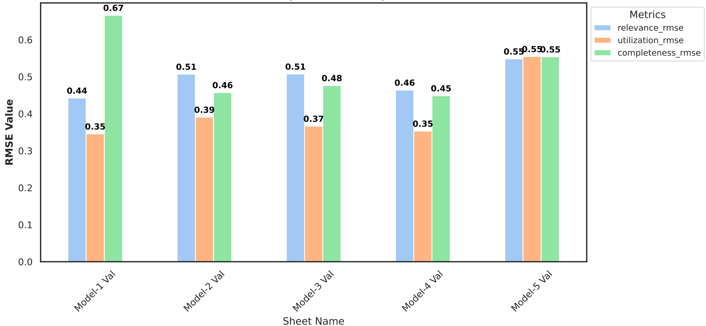
RMSE Comparison (Val Split)
