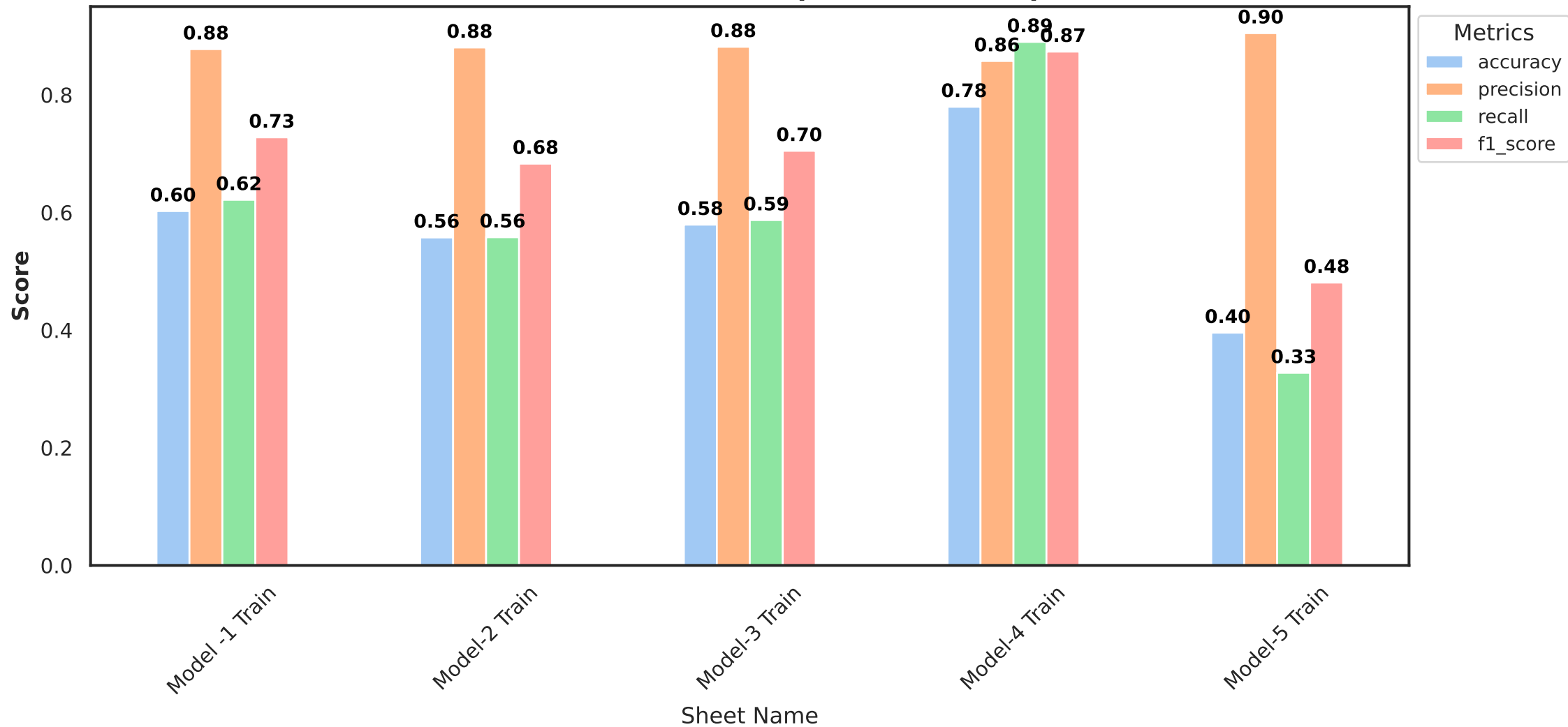
Classification Metrics Comparison (Train Split)
