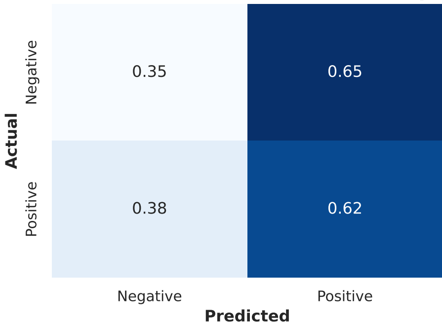
Confusion Matrix - Model-5 Val (Val Split)
