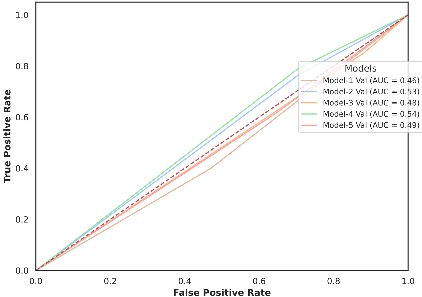
ROC Curves for Adherence Score (Val Split)
