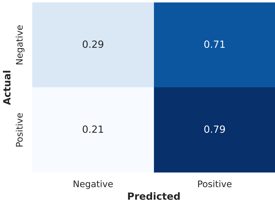
Confusion Matrix - Model-4 Val (Val Split)
