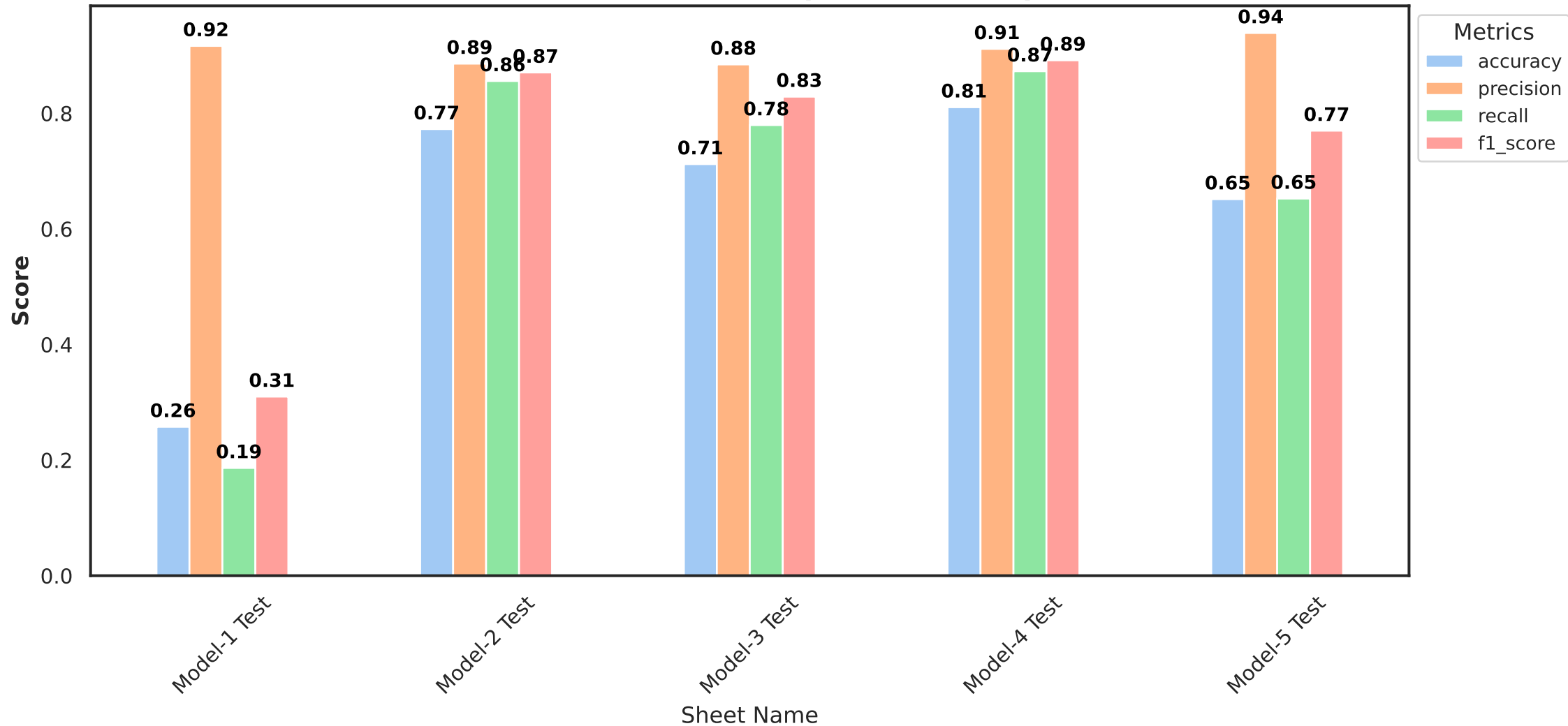
Classification Metrics Comparison (Test Split)
