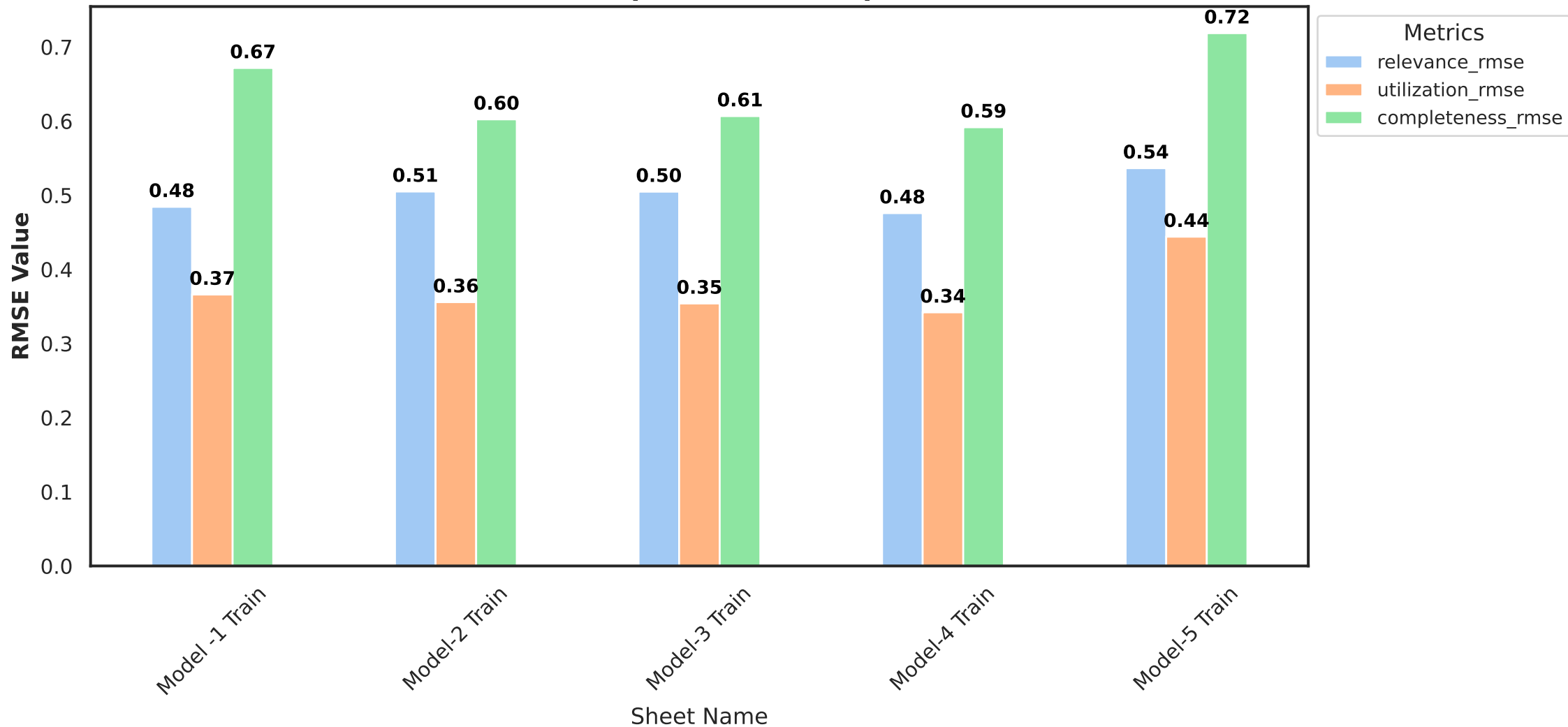
RMSE Comparison (Train Split)
