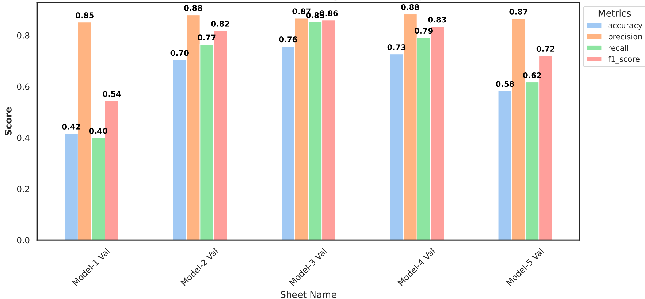
Classification Metrics Comparison (Val Split)
