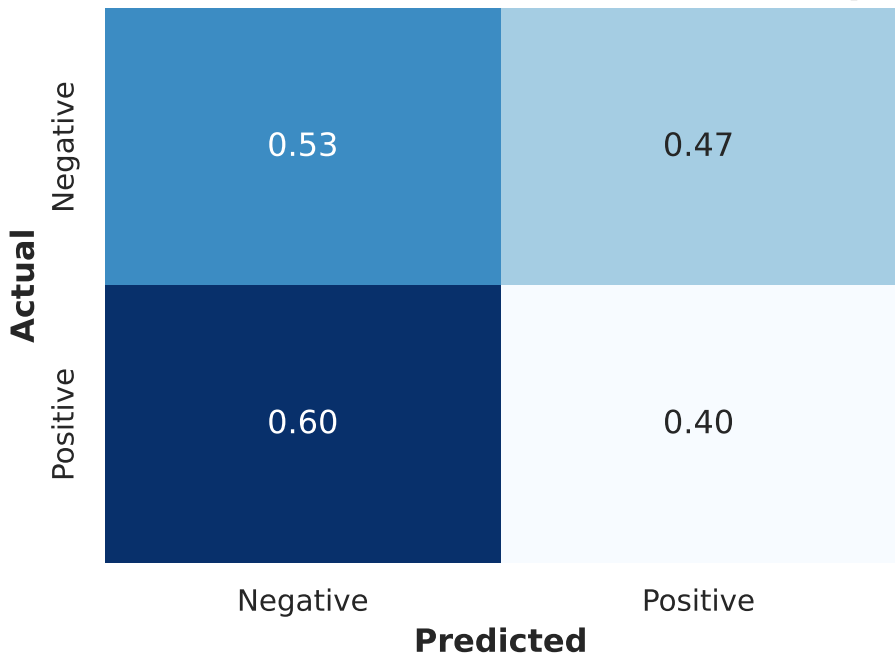
Confusion Matrix - Model-1 Val (Val Split)
